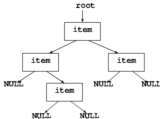
Figure 15.4: Binary tree. The top node is the root node. Each node contains an item of data and has two links to child nodes, which may point to NULL . In this figure, the bottom and righthand nodes are leaf nodes.
