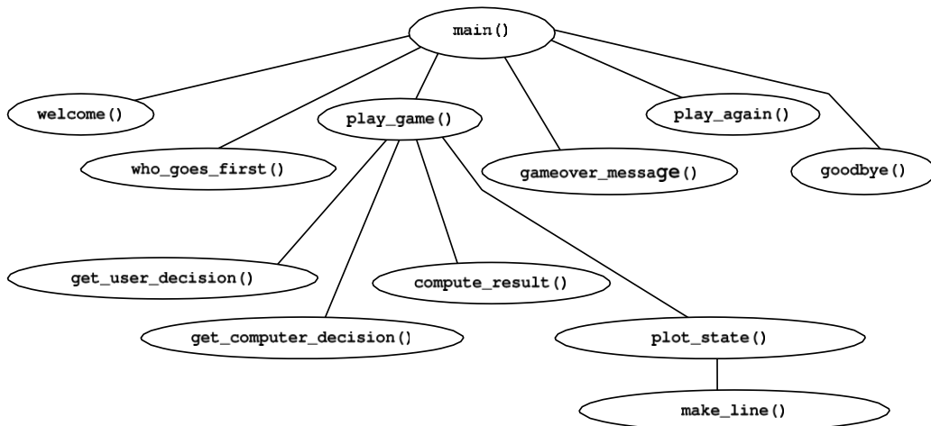
Figure 6.3: The top-down design of the Tic-Tac-Toe program.
